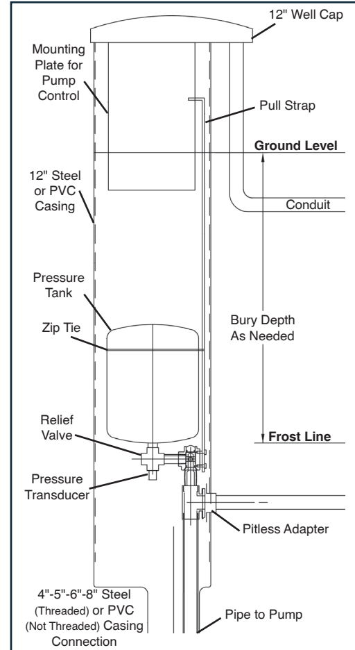
PCM for Variable Speed Pump Steel or PVC Casing
